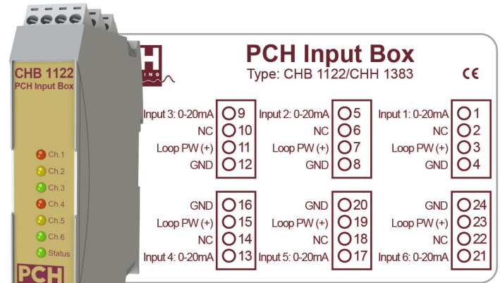
Example: 6 of 4-20 mA Inputs with Loop Power
